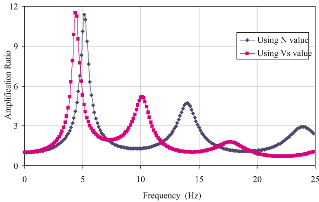
Figure 15. Typical amplification ratio using MASW and SPT.
