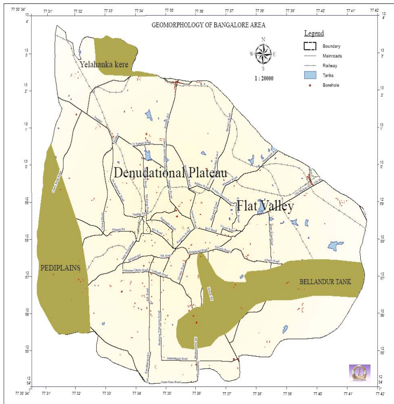
Figure 2. Geomorphology of Bangalore area.
